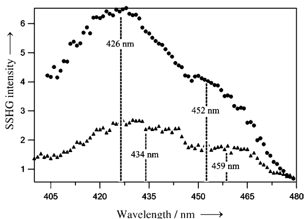
Figure 2. SSHG spectra of 50 \mu\text{m} (▲) and 100 \mu\text{m} (●) [\text{CoTMPyP}]^{4+} (P) recorded at the [\text{water}|\text{DCE}(\text{TB}^-)] interface.
