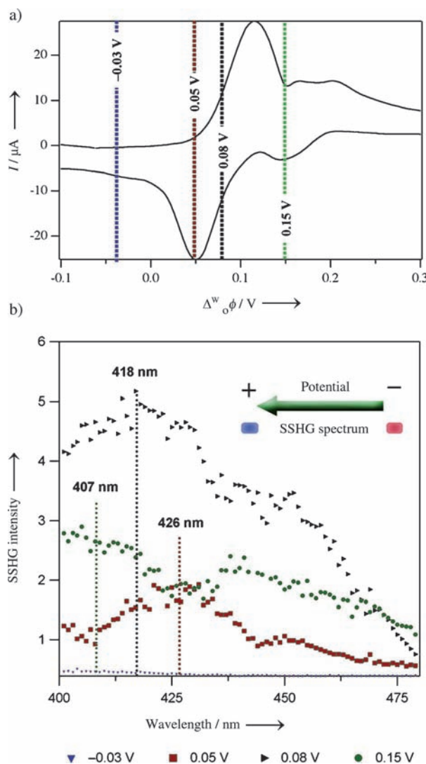
Figure 3. a) Ion-transfer voltammogram of 50 \mu\text{m} [\text{CoTMPyP}]^{4+} at neutral pH (sweep rate 50 \text{mVs}^{-1} ). b) SSHG spectra of 50 \mu\text{m} [\text{CoTMPyP}]^{4+} recorded under polarization of the interface by using a four-electrode system.
