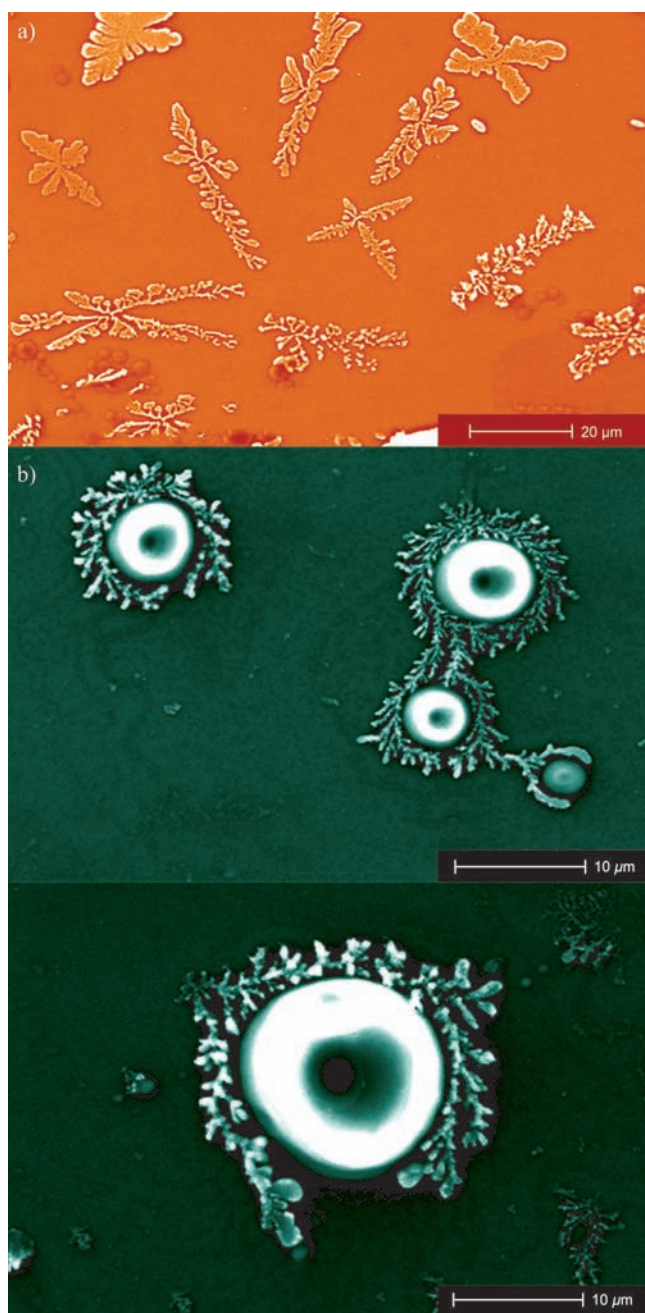
Figure 4. Secondary-electron SEM images (10 kV) of [\text{CoTMPyP}]^{4+} at the a) [\text{water}|\text{DCE}] and b) [\text{water}|\text{DCE}(\text{TB}^-)] interfaces.
